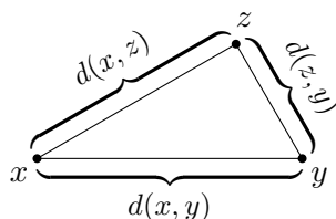
Figure 1. The triangle inequality: d(x, y) \leq d(x, z) + d(z, y) .
