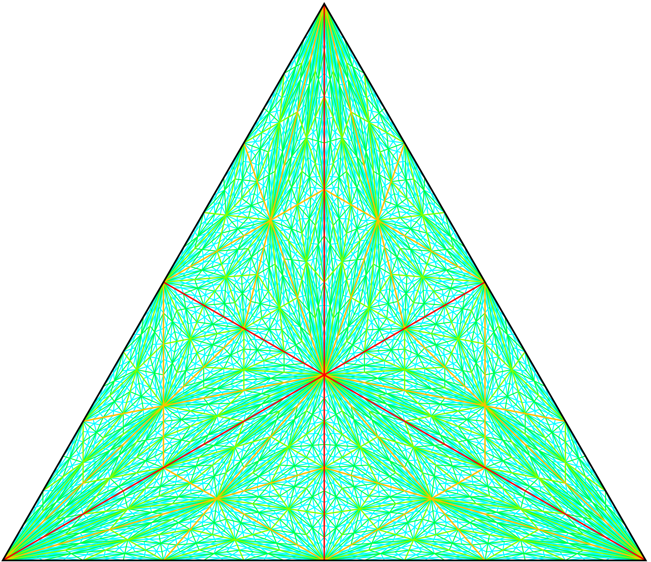
Fifth barycentric subdivision
