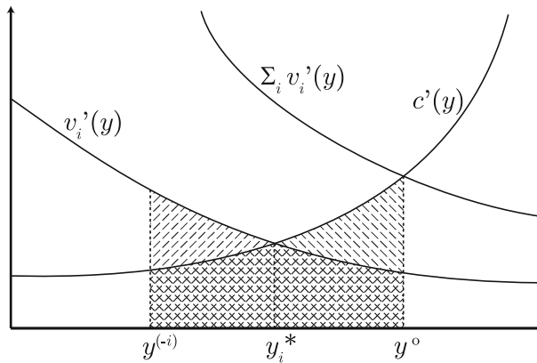
Fig. 5 The largest y^{(-i)} such that the Pareto optimal public good level y^o satisfies EP_i
