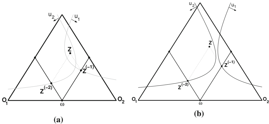
Fig. 2 Opt-out allocations z^{(-1)} and z^{(-2)} where the original point z is preferred by both agents (a), and where one agent prefers to opt out (b)
