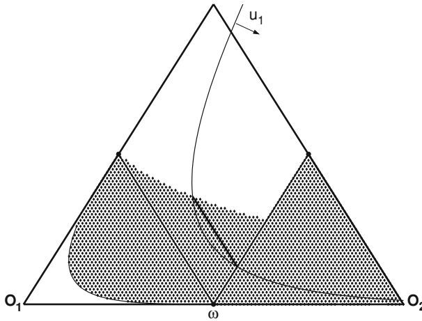
Fig. 3 An example of the set \mathcal{EP}_1(e) for a two-agent economy with convex preferences
