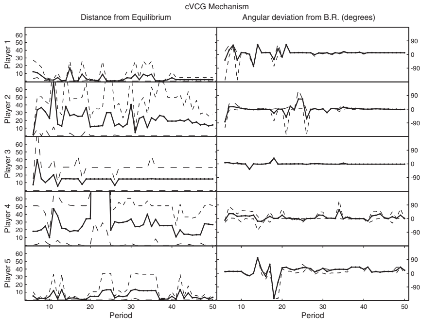
Fig. 11. Time series of average distance from equilibrium and angular deviation from the best response line for each player type in the cVCG mechanism with 95% confidence intervals.
