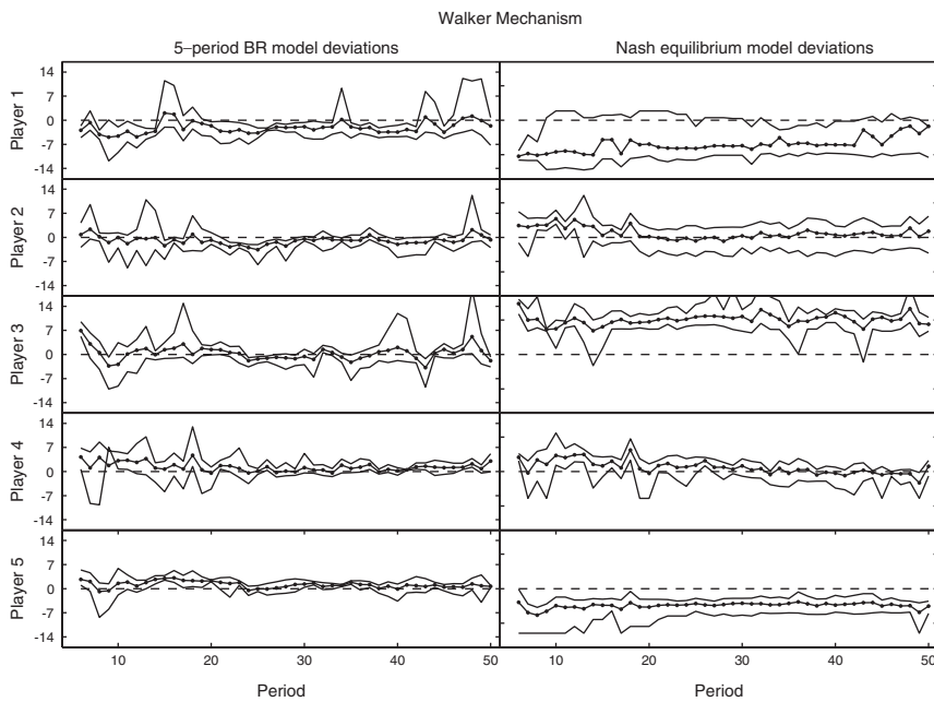
Fig. 4. Average model error for the 5-period best response model and Nash equilibrium models in the Walker mechanism.
