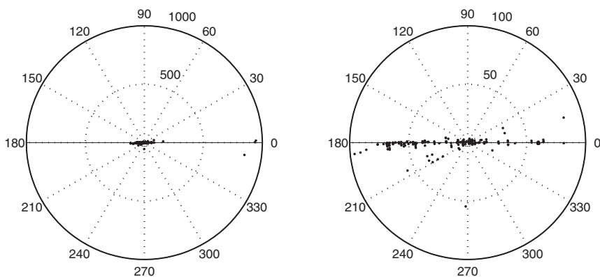
Fig. 10. Polar-coordinate representation of the cVCG data with the origin at the truth-telling point and the horizontal axis corresponding to the 5-period best response surface. Two different scalings of the same graph are presented.
