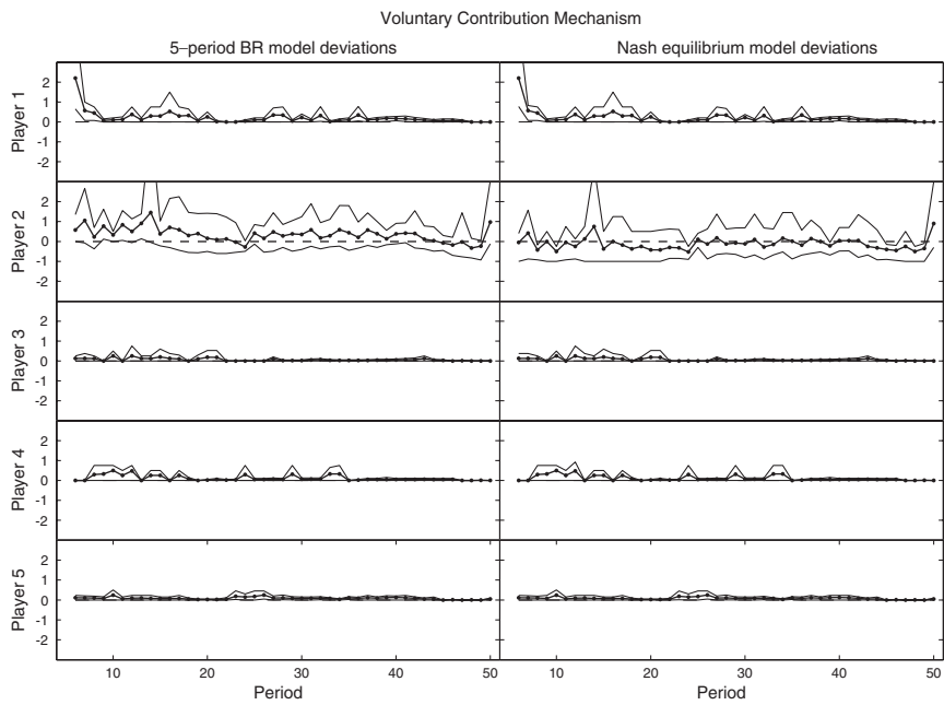
Fig. 1. Average model error for the 5-period best response model and Nash equilibrium models in the Voluntary Contribution mechanism.
