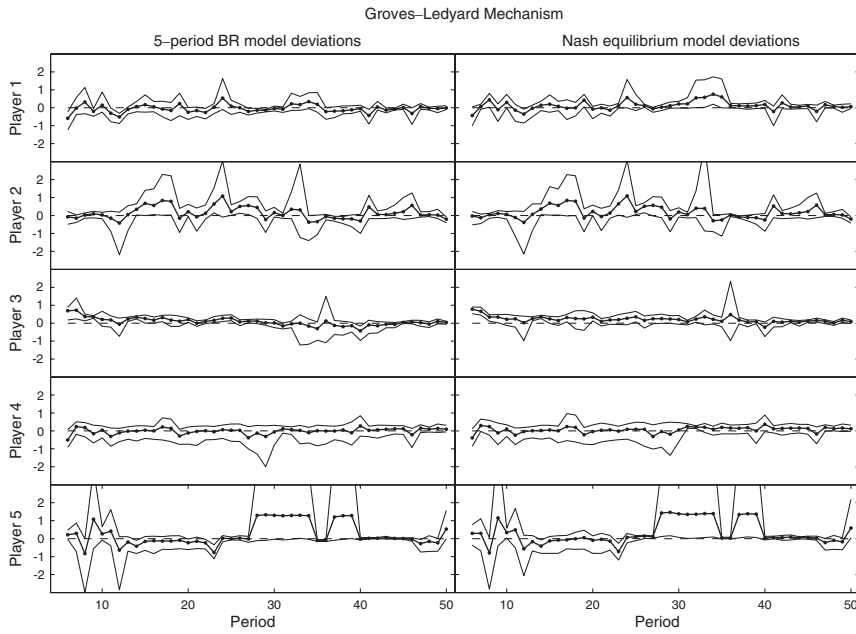
Fig. 3. Average model error for the 5-period best response model and Nash equilibrium models in the Groves–Ledyard mechanism.
