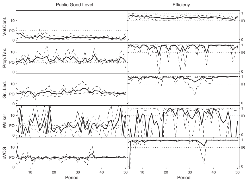
Fig. 12. The average level of public good and realized efficiency for each mechanism in each period along with 95% confidence intervals. PO represents the Pareto Optimal level of the public good (4.8095) and IR represents the efficiency of the initial endowments (71.18%).
