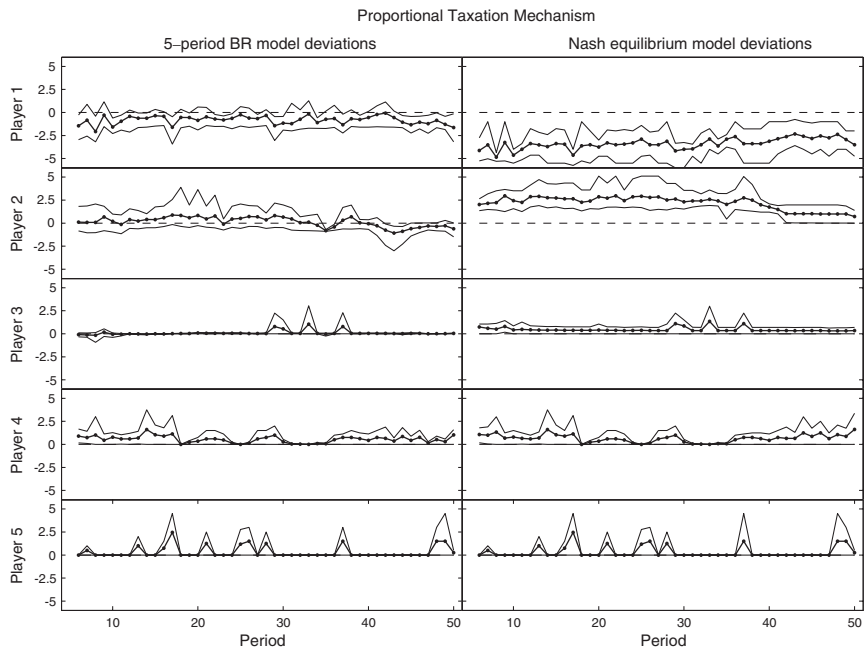
Fig. 2. Average model error for the 5-period best response model and Nash equilibrium models in the Proportional Taxation mechanism.
